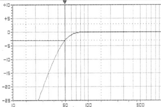
PREDICTED LOW FREQUENCY RESPONSE • Bass-reflex cabinet, Vb=80 l, fb=45 Hz.
